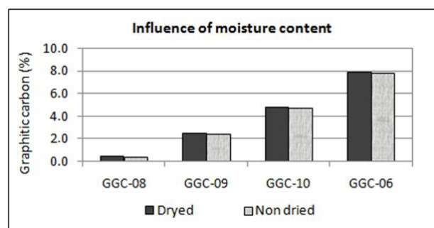
Figure 1. Influence of moisture content in graphitic carbon results.
