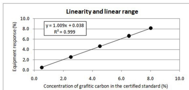
Figure 5. Linearity and linear working range for graphitic carbon optimized method.
