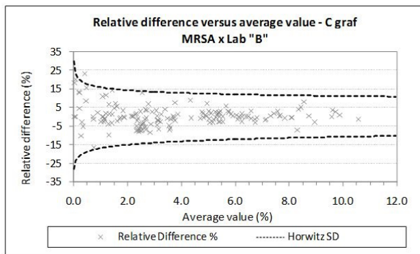
Figure 7. Comparison between results of graphitic carbon reported by MRSA and commercial laboratory “B” – Horwitz analysis.
