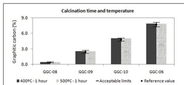
Figure 4. Influence of calcination time and temperature in graphitic carbon results.
