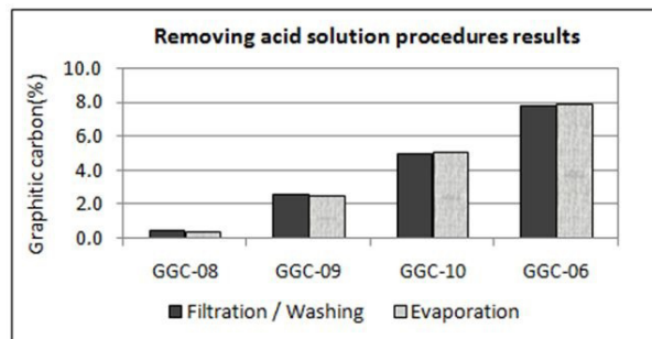
Figure 2. Influence of HCl filtration/washing and evaporation in graphitic carbon results.
