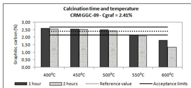
Figure 3. Influence of calcination time and temperature in graphitic carbon results for CRM GGC-09
